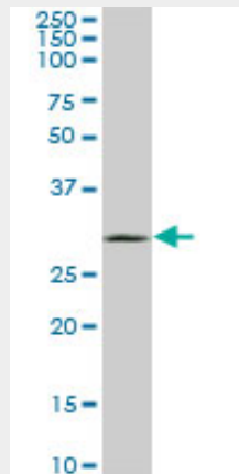
UCP1 monoclonal antibody (M03), clone 4B7. Western Blot analysis of UCP1 expression in NIH/3T3 ( (Cat # AT4459a )
