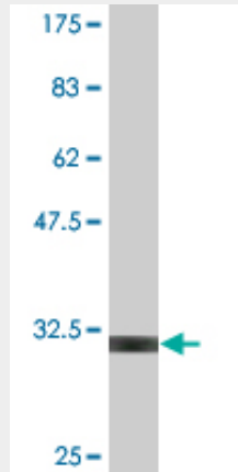
Antibody Reactive Against Recombinant Protein. Western Blot detection against Immunogen (29.7 KDa) .
