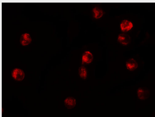
Immunofluorescence of JMJD3 in K562 cells with JMJD3 antibody at 20 µg/mL.
