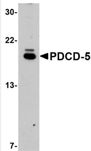
Western blot analysis of PDCD5 in EL4 cell lysate with PDCD5 antibody at 1 \mu g/mL.
