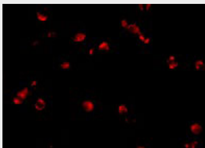
Immunofluorescence of PDCD5 in Jurkat cells with PDCD5 antibody at 10 \mu g/mL.
