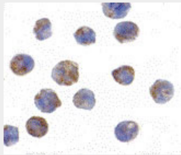
Immunocytochemistry of PHAP I in Raji cells with PHAP I antibody at 2 \mu\text{g/mL} .
