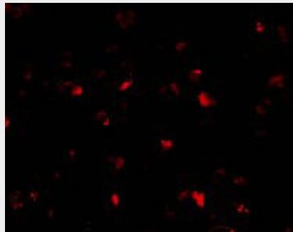
Immunofluorescence of PHAP I in Raji cells with PHAP I antibody at 10 \mu\text{g/mL} .
