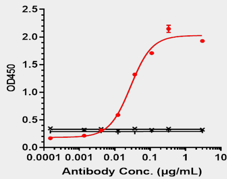
Monkeypox Virus (strain Zaire-96-I-16) A35R, mFc Tag at 2 ug/mL can bind Anti-Monkeypox Virus Antibody, The EC50 is 0.02820 ug/mL.
