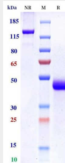
Monkeypox Virus (strain Zaire-96-I-16) A35R, mFc Tag on SDS-PAGE under reducing (R) and Non-reducing (NR) condition. The purity of the protein is greater than 85%.
