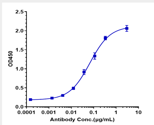
Immobilized human IGF1R His at 2 µg/mL can bind Anti-IGF1R / CD221 Reference Antibody (lonigutamAb) EC_{50}=0.06727 µg/mL
