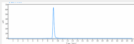
The purity of Anti-IGF1R / CD221 Reference Antibody (lonigutamAb) is more than 100%, determined by SEC-HPLC.
