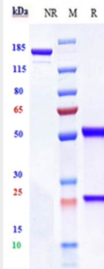
Anti-IGF1R / CD221 Reference Antibody (lonigutamAb) on SDS-PAGE under reducing (R) condition. The gel was stained with Coomassie Blue. The purity of the protein is greater than 95%
