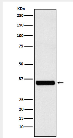
Western blot analysis of EXOSC7 expression in Jurkat cell lysate.
