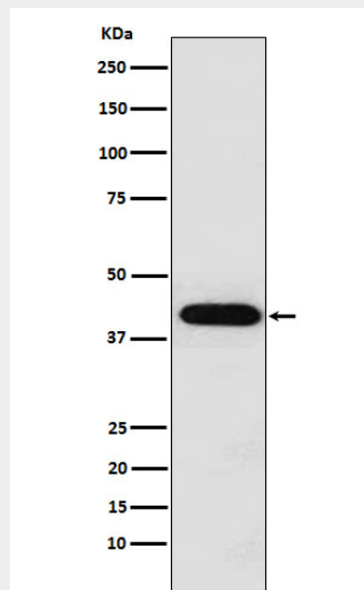
Western blot analysis of Inhibin alpha expression in HeLa cell lysate.
