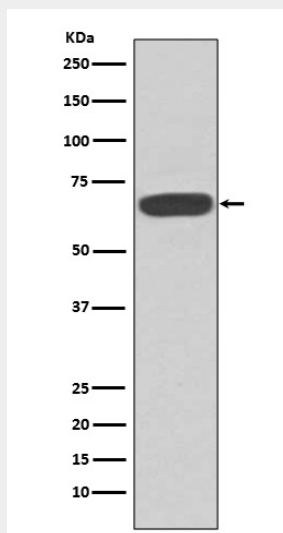
Western blot analysis of PKR expression in MCF-7 cell lysate.
