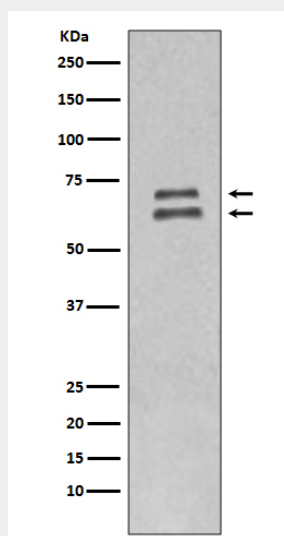
Western blot analysis of Lamin A/C expression in HeLa whole cell lysates.
