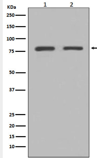
Western blot analysis of GRP78 BiP expression in (1) HeLa cell lysate; (2) C6 cell lysate.
