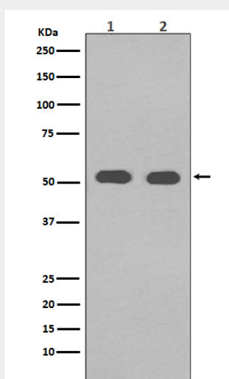
Western blot analysis of alpha Tubulin in (1) HeLa cell lysate; (2) NIH/3T3 cell lysate.
