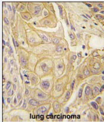
Formalin-fixed and paraffin-embedded human lung carcinoma tissue reacted with EphB2 antibody (Cat.#AP7623d), which was peroxidase-conjugated to the secondary antibody, followed by DAB staining. This data demonstrates the use of this antibody for immunohistochemistry; clinical relevance has not been evaluated.
