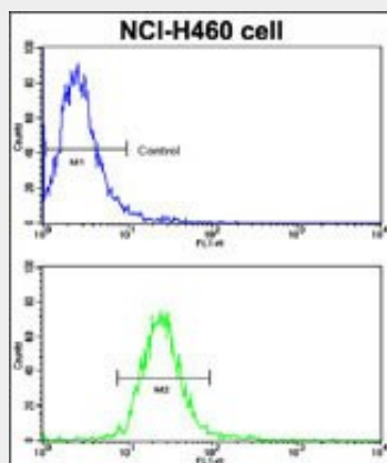
Flow cytometric analysis of NCI-H460 cells using EphB2 Antibody (bottom histogram) compared to a negative control cell (top histogram). FITC-conjugated goat-anti-rabbit secondary antibodies were used for the analysis.
