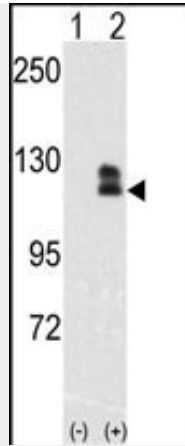
Western blot analysis of EphB2 (arrow) using rabbit polyclonal EphB2 Antibody (Cat.#AP7623d). 293 cell lysates (2 ug/lane) either nontransfected (Lane 1) or transiently transfected with the EphB2 gene (Lane 2) (Origene Technologies).
