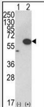
Western blot analysis of AKT1 (arrow) using rabbit polyclonal hAKT1-D453 (Cat. #AP7028b). 293 cell lysates (2 ug/lane) either nontransfected (Lane 1) or transiently transfected with the AKT1 gene (Lane 2) (Origene Technologies).
