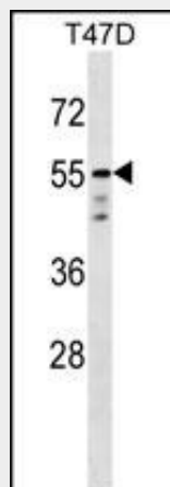
AKT1 Antibody (C-term) (Cat. #AP7028b) western blot analysis in T47D cell line lysates (35ug/lane).This demonstrates the AKT1 antibody detected the AKT1 protein (arrow).
