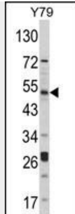
Western blot analysis of hAKT1-D453 (Cat. #AP7028b) in Y79 cell line lysates (35ug/lane).AKT1 (arrow) was detected using the purified Pab.
