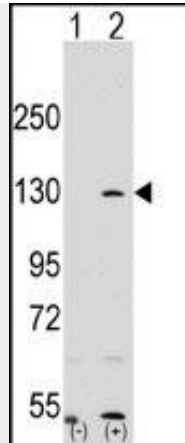
Western blot analysis of PARP1 (arrow) using rabbit polyclonal PARP1 Antibody (N-term)(Cat.#AP6373a). 293 cell lysates (2 ug/lane) either nontransfected (Lane 1) or transiently transfected with the PARP1 gene (Lane 2) (Origene Technologies).
