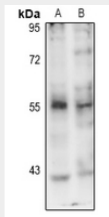
Western blot analysis of PINK1 (pS402) expression in MCF7 (A), HCT116 (B) whole cell lysates.
