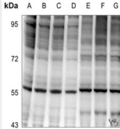
Western blot analysis of NF-kappaB p65 (pT254) expression in MCF7-LPS-30mins (A), MCF7-LPS-15mins (B), MCF7-LPS-5mins (C), MCF7 (D), Hela-TNFa-15mins (E), Hela-TNFa-5mins (F), Hela (G) whole cell lysates.
