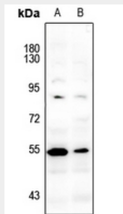
Western blot analysis of LCK (pY393) expression in Myla2059 (A), HuT78 (B) whole cell lysates.
