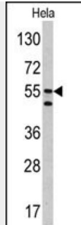
Western blot analysis of CA9 antibody (Center) (Cat.# AP5000e) in HeLa cell line lysates (35ug/lane). CA9 (arrow) was detected using the purified Pab.
