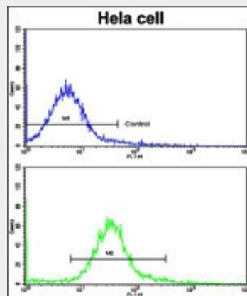
Flow cytometric analysis of heLa cells using CA9 Antibody (Center)(bottom histogram) compared to a negative control cell (top histogram). FITC-conjugated goat-anti-rabbit secondary antibodies were used for the analysis.
