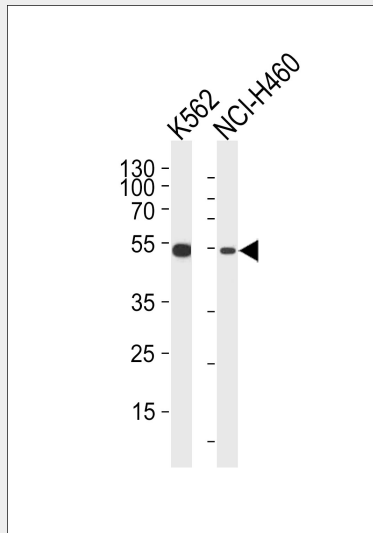
CHEK2 Antibody (N-term) (Cat. #AP4999a) western blot analysis in K562,NCI-H460 cell line lysates (35ug/lane).This demonstrates the CHEK2 antibody detected the CHEK2 protein (arrow).
