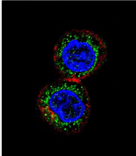
Confocal immunofluorescent analysis of CHEK2 Antibody (N-term)(Cat#AP4999a) with HepG2 cell followed by Alexa Fluor 488-conjugated goat anti-rabbit IgG (green).Actin filaments have been labeled with Alexa Fluor 555 phalloidin (red).DAPI was used to stain the cell nuclear (blue).
