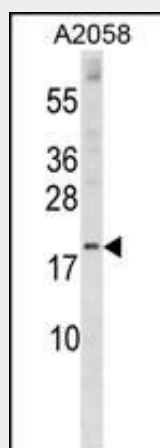
SNX3 Antibody (Center) (Cat. #AP18477c) western blot analysis in A2058 cell line lysates
