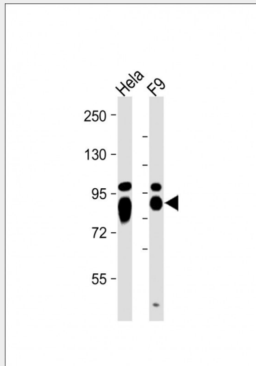
All lanes : Anti-ALPL Antibody (Center) at 1:2000 dilution Lane 1: HeLa whole cell lysate Lane 2: F9 whole cell lysate Lysates/proteins at 20 µg per lane. Secondary Goat Anti-Rabbit IgG, (H+L), Peroxidase conjugated at 1/10000 dilution. Predicted band size : 57 kDa Blocking/Dilution buffer: 5% NFDM/TBST.
