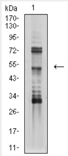
Figure 3: Western blot analysis using TFAP2B mAb against HEK293 (1) and TFAP2B (AA: 84-193)-hlgGfc transfected HEK293 (2) cell lysate.
