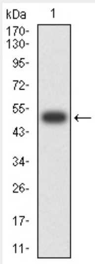
Western blot analysis using MIB1 mAb against human MIB1 (AA: 6-221) recombinant protein. (Expected MW is 50.1 kDa)
