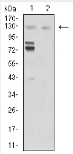
Western blot analysis using MIB1 mAb against HEK293 (1) and MIB1 (AA: 6-221)-hlgGfC transfected HEK293 (2) cell lysate.
