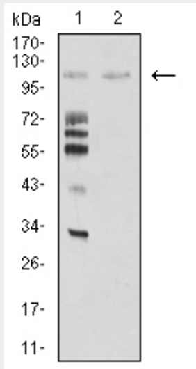
Western blot analysis using MIB1 mAb against HEK293 (1) and MIB1 (AA: 6-221)-hIgGfC transfected HEK293 (2) cell lysate.
