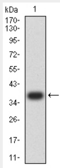
Western blot analysis using SMAD1 mAb against human SMAD1 (AA: 1-110) recombinant protein. (Expected MW is 38.5 kDa)
