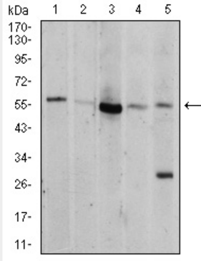
Western blot analysis using AKT1 mouse mAb against MCF-7 (1), NIH/3T3 (2), HeLa (3), COS7 (4), and C6 (5) cell lysate.
