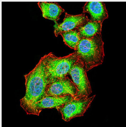
Immunofluorescence analysis of HepG2 cells using AKT1 mouse mAb (green). Blue: DRAQ5 fluorescent DNA dye. Red: Actin filaments have been labeled with Alexa Fluor- 555 phalloidin.
