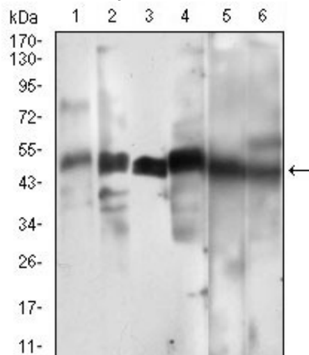
Figure 2: Western blot analysis using CCNA2 mAb against HEK293 (1) and CCNA2 (AA: 105-233)-hlgGfc transfected HEK293 (2) cell lysate.
