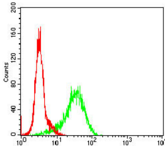
Figure 2: Flow cytometric analysis of NIH/3T3 cells using GSK3B mouse mAb (green) and negative
