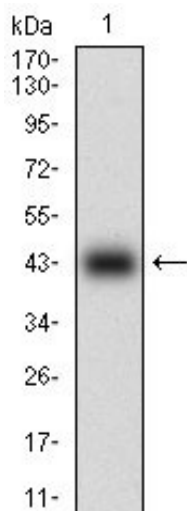
Figure 1: Western blot analysis using CAV2 mAb against human CAV2 (AA: 1-86) recombinant protein. (Expected MW is 35.9 kDa)
