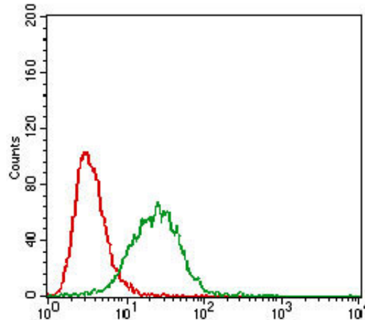
Figure 4: Flow cytometric analysis of A549 cells using CAV2 mouse mAb (green) and negative control (red).
