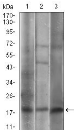
Figure 2: Western blot analysis using CAV2 mAb against HEK293 (1) and CAV2 (AA: 1-86)-hlgGfC transfected HEK293 (2) cell lysate.
