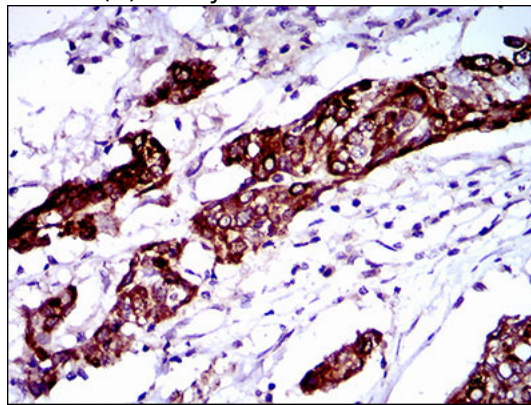
Figure 3: Immunohistochemical analysis of paraffin-embedded esophagus cancer tissues using BRCA1 mouse mAb with DAB staining.
