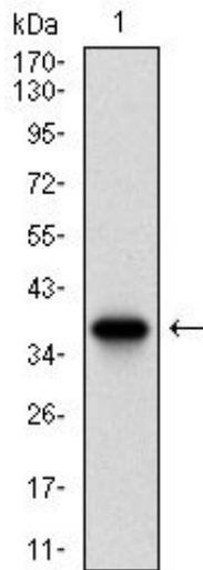
Figure 1: Western blot analysis using BRCA1 mAb against human BRCA1 recombinant protein. (Expected MW is 37.5 kDa)
