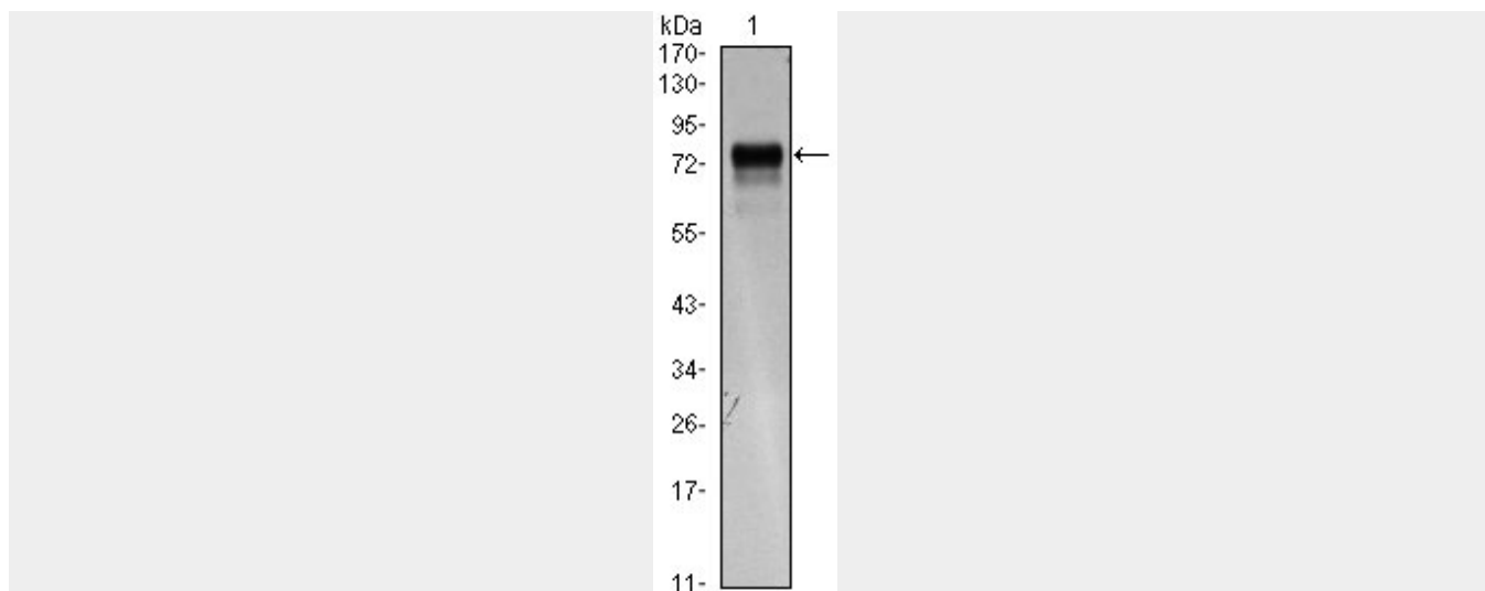
Figure 1: Western blot analysis using FLT4 mAb against FLT4(AA: 25-330)-hlgGfc transfected HEK293 cell lysate.
