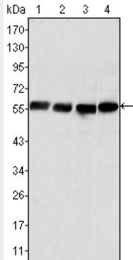
Figure 1: Western blot analysis using Vimentin mouse mAb against HeLa (1), COS (2), HEK293 (3) and U2OS (4) cell lysate.
