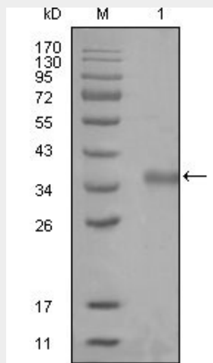
Figure 1: Western blot analysis using NCOR1 mouse mAb against truncated Trx-NCOR1
