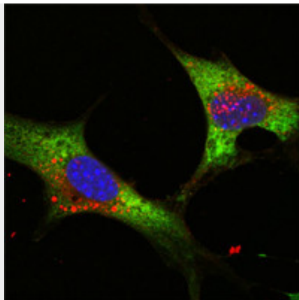
Figure 3: Confocal immunofluorescence analysis of NTERA-2 cells using anti-LIN28 mAb (green). Blue: DRAQ5 fluorescent DNA dye.
