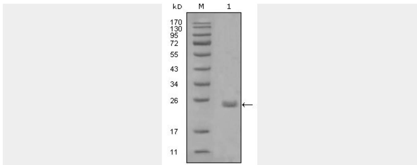
Figure 1: Western blot analysis using AXL mouse mAb against truncated Trx-AXL recombinant protein (1).
