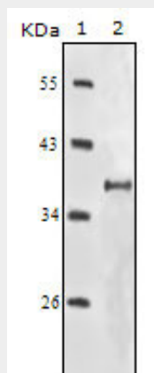
Figure 1: Western blot analysis using IGF1R-Beta mouse mAb against truncated IGF1R-Beta recombinant protein.
