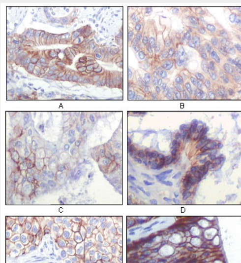
Figure 2: Immunohistochemical analysis of paraffin-embedded human gastric adenocarcinoma(A), colon adenocarcinoma(B), endometrial carcinoma(uterus)(C), ovary adenocarcinoma(D), lung squamous cell carcinoma(E), stomach epithelium mucosae(F), showing membrane localization using IGF1R-Beta mouse mAb with DAB staining.
