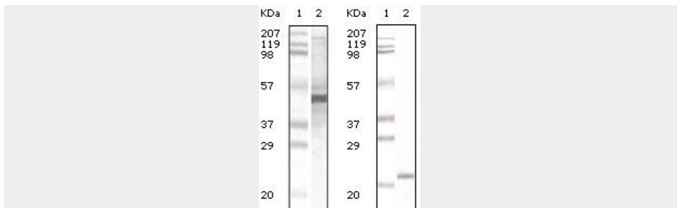
Figure 2: Western blot analysis using ApoA5 mouse mAb against human serum (A) and ApoA5 recombinant protein (B).
