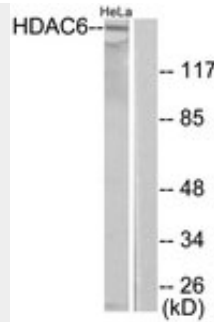
Western blot of extracts from HeLa cells, using HDAC6 Antibody.
