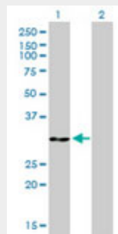
Western blot of ANXA5 expression in transfected 293T cell line by ANXA5 monoclonal antibody...
