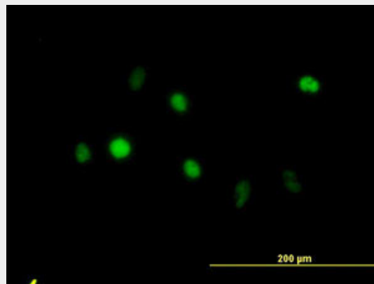
Immunofluorescence of monoclonal antibody to ANXA5 on HeLa cell. [antibody concentration 10 ug/ml]
