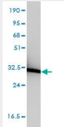
ANXA5 monoclonal antibody (M01), clone 1F4-1A5 Western blot of ANXA5 expression in HeLa.
