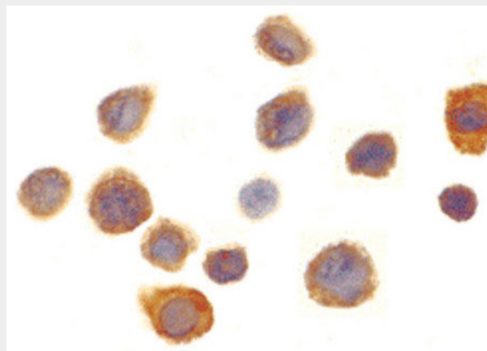
Immunocytochemistry of SIRP alpha in THP-1 cells with SIRP alpha antibody at 1 ug/ml.
