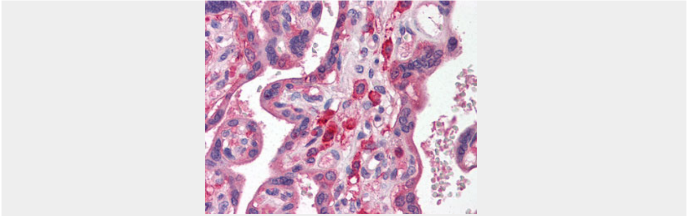
Anti-SIRPA antibody IHC of human placenta.
