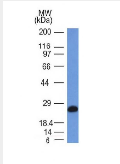
Western Blot of Ramos Cell Lysate using CD79a Monoclonal Antibody (IGA/1406).
