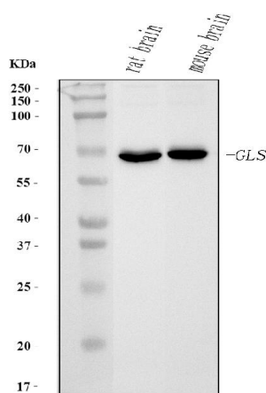
Figure 2. Western blot analysis of Glutaminase/GLS using anti-Glutaminase/GLS antibody (M01272-2).
