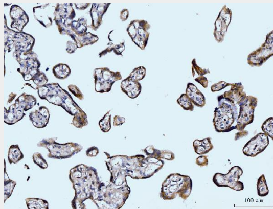
Figure 6. IHC analysis of Glutaminase/GLS using anti-Glutaminase/GLS antibody (M01272-2). Glutaminase/GLS was detected in a paraffin-embedded section of human placenta tissue. Heat mediated antigen retrieval was performed in EDTA buffer (pH 8.0, epitope retrieval solution). The tissue section was blocked with 10% goat serum. The tissue section was then incubated with 2 μg/ml mouse anti-Glutaminase/GLS Antibody (M01272-2) overnight at 4°C. Biotinylated goat anti-mouse IgG was used as secondary antibody and incubated for 30 minutes at 37°C. The tissue section was developed using Streptavidin-Biotin-Complex (SABC) (Catalog # SA1021) with DAB as the chromogen.
