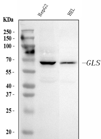
Figure 1. Western blot analysis of Glutaminase/GLS using anti-Glutaminase/GLS antibody (M01272-2).
