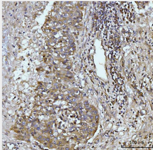
Figure 5. IHC analysis of Glutaminase/GLS using anti-Glutaminase/GLS antibody (M01272-2). Glutaminase/GLS was detected in a paraffin-embedded section of human liver cancer tissue. Heat mediated antigen retrieval was performed in EDTA buffer (pH 8.0, epitope retrieval solution). The tissue section was blocked with 10% goat serum. The tissue section was then incubated with 2 μg/ml mouse anti-Glutaminase/GLS Antibody (M01272-2) overnight at 4°C. Biotinylated goat anti-mouse IgG was used as secondary antibody and incubated for 30 minutes at 37°C. The tissue section was developed using Streptavidin-Biotin-Complex (SABC) (Catalog # SA1021) with DAB as the chromogen.
