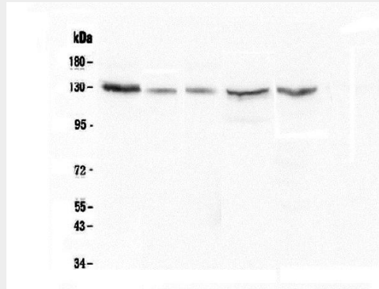
Figure 2. Western blot analysis of CASR using anti-CASR antibody (M00574). Electrophoresis was performed on a 8% SDS-PAGE gel at 70V (Stacking gel) / 90V (Resolving gel) for 2-3 hours. The sample well of each lane was loaded with 50ug of sample under reducing conditions.
