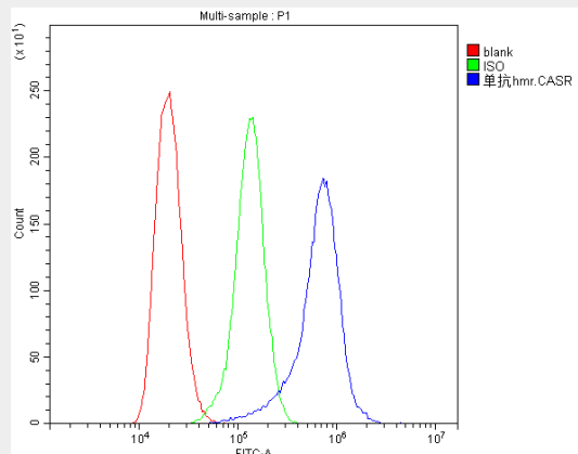
Figure 1. Flow Cytometry analysis of NEURO-2A cells using anti-CASR antibody (M00574).
