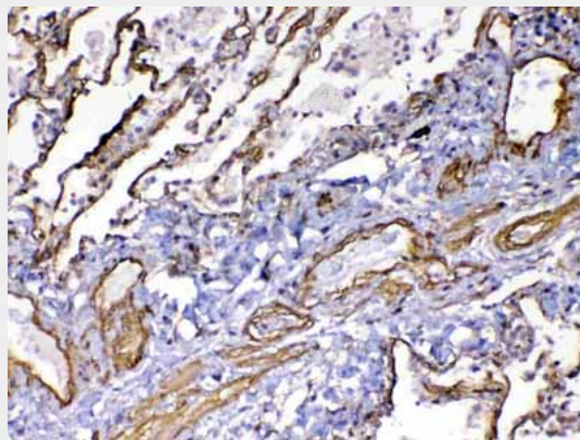
Figure 2. IHC analysis of VEGF Receptor 3 using anti-VEGF Receptor 3 antibody (ABO12937). VEGF Receptor 3 was detected in paraffin-embedded section of human lung cancer tissue. Heat mediated antigen retrieval was performed in citrate buffer (pH6, epitope retrieval solution) for 20 mins. The tissue section was blocked with 10% goat serum. The tissue section was then incubated with 1 \mu g/ml rabbit anti-VEGF Receptor 3 Antibody (ABO12937) overnight at 4 ^{\circ} C. Biotinylated goat anti-rabbit IgG was used as secondary antibody and incubated for 30 minutes at 37 ^{\circ} C. The tissue section was developed using Streptavidin-Biotin-Complex (SABC) with DAB as the chromogen.
