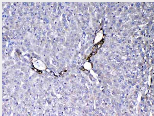
Figure 4. IHC analysis of VEGF Receptor 3 using anti-VEGF Receptor 3 antibody (ABO12937).
