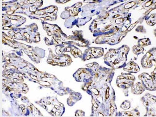
Figure 3. IHC analysis of VEGF Receptor 3 using anti-VEGF Receptor 3 antibody (ABO12937). VEGF Receptor 3 was detected in paraffin-embedded section of human placenta tissue. Heat mediated antigen retrieval was performed in citrate buffer (pH6, epitope retrieval solution) for 20 mins. The tissue section was blocked with 10% goat serum. The tissue section was then incubated with 1 \mu g/ml rabbit anti-VEGF Receptor 3 Antibody (ABO12937) overnight at 4 ^{\circ} C. Biotinylated goat anti-rabbit IgG was used as secondary antibody and incubated for 30 minutes at 37 ^{\circ} C. The tissue section was developed using Streptavidin-Biotin-Complex (SABC) with DAB as the chromogen.
