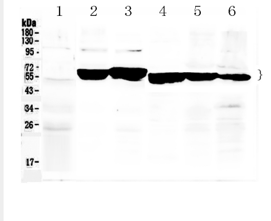
Figure 1. Western blot analysis of Cytokeratin 8 using anti- Cytokeratin 8 antibody (ABO10184). Electrophoresis was performed on a 5-20% SDS-PAGE gel at 70V (Stacking gel) / 90V (Resolving gel) for 2-3 hours. The sample well of each lane was loaded with 50ug of sample under reducing conditions. Lane 1: rat liver tissue lysates, Lane 2: mouse ovary tissue lysates, Lane 3: mouse liver tissue lysates, Lane 4: MCF-7 whole cell lysates, Lane 5: A549 whole cell lysates, Lane 6: HELA whole Cell lysates. After Electrophoresis, proteins were transferred to a Nitrocellulose membrane at 150mA for 50-90 minutes. Blocked the membrane with 5% Non-fat Milk/ TBS for 1.5 hour at RT. The membrane was incubated with rabbit anti- Cytokeratin 8 antigen affinity purified polyclonal antibody (Catalog # ABO10184) at 0.5 \mu g/mL overnight at 4 ^{\circ} C, then washed with TBS-0.1% Tween 3 times with 5 minutes each and probed with a goat anti-rabbit IgG-HRP secondary antibody at a dilution of 1:10000 for 1.5 hour at RT. The signal is developed using an Enhanced Chemiluminescent detection (ECL) kit with Tanon 5200 system. A specific band was detected for Cytokeratin 8 at approximately 54KD, 56KD. The expected band size for Cytokeratin 8 is at 54KD.
